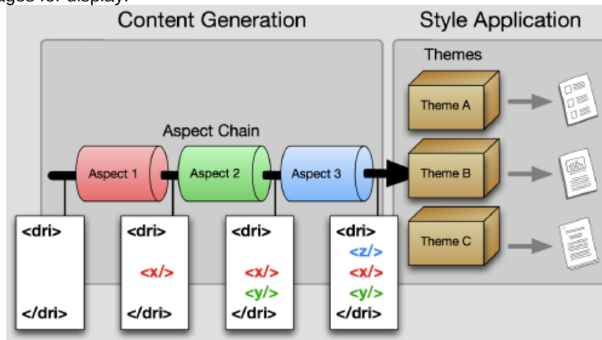
Figure 1: The Manakin Architecture
