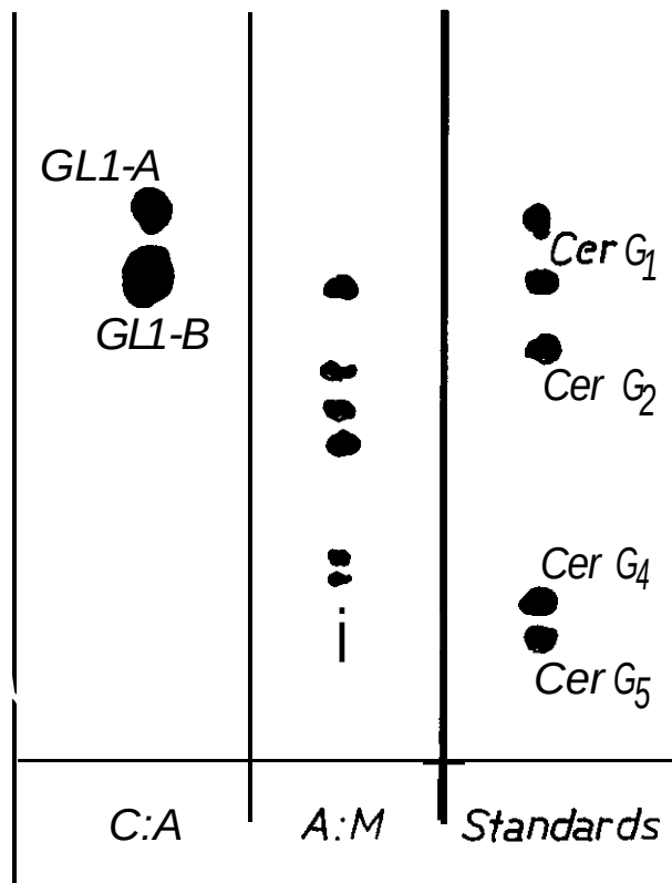
Figure 1. Thin layer chromatography (Silica gel G, Merck) of lipids in fractions C:A and A:M from a silicic acid column. The solvent was chloroform:methanol:water (65:25:4,v:v:v). The plate was stained with the orcinol reagent. CerG 1 , CerG 2 , CerG 4 , and CerG 5 , standards of mono, di, tetra and pentahexosyl ceramide (Supelco).
