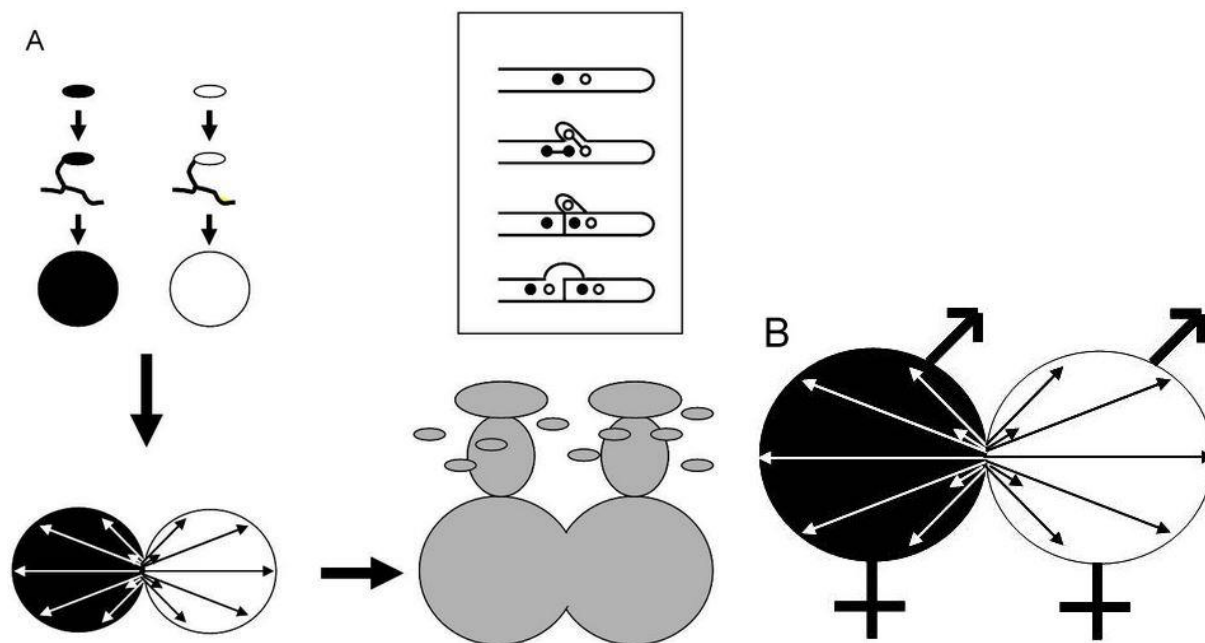
Figure 1. The standard life cycle of a heterothallic basidiomycete fungus. Sexual spores germinate (upper left) give rise to a haploid monokaryon. Two compatible monokaryons can fuse, upon which they reciprocally exchange nuclei, without cytoplasmic mixing (down left). This leads to the formation of the dikaryon (grey, right), all cells of which have two different nuclei, and which
