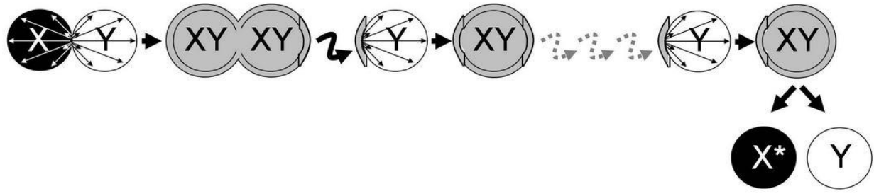
Figure 2. Experimental set-up for artificial selection for fast migration of nucleus X . Nucleus X is serially passed through monokaryon Y , which is not coevolving. This experimental set-up uses the 'Buller phenomenon', since the newly formed dikaryon XY fertilizes monokaryon Y . At the end of the experiment, the nuclear migration rate of the evolved X can be compared with that of the ancestral X .
