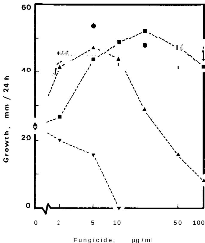
Figure 1. -- Effect of fungicides on growth of N. crassa mutant smco-2 . Each point is the mean growth rate (increase in colony diameter at 26°C) of at least 3 replicates on MM containing dicloran ▲; iprodione ▼; vinclozolin ■; or quintozone ●
