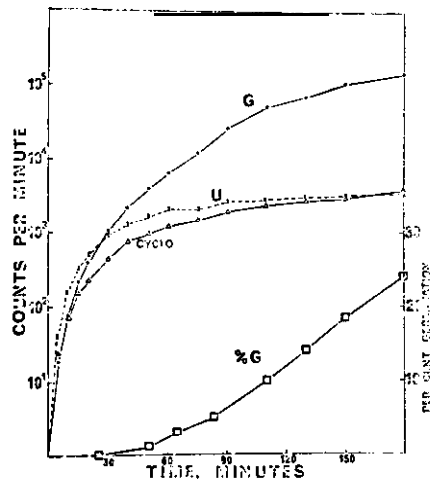
Figure 1. The effect of cycloheximide on RNA synthesis. Incorporation of uracil-2- C^{14} (5 \mu c/flask, 0.075 mM) into TCA insoluble material. G="germinating"; U="non-germinating"; CYCLO=cycloheximide, 100 \mu g/ml; % G= percent germination of "germinating" conidia.
