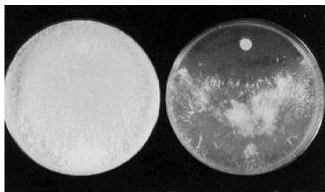
Fig. 1. Assay method. Wild type (left) and sod-1 (right) strains were inoculated onto Vogel's N medium opposite a Whatman #1 filter-paper disk that had been dipped in 500 mM paraquat. The plates were photographed after several days growth at room temperature.
