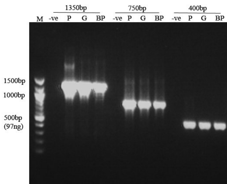
Figure 1. Comparison of PCR amplicons from Boil-prep genomic DNA (BP), genomic DNA (G) (prepared by the method of Ireland et al. 1993), plasmid DNA (P) and no DNA (-ve) templates. Size marker (M) = 100bp DNA ladder (New England Biolabs) with a 500bp reference band that contains 97ng of DNA. Each sample lane contains 6ul of a 50ul PCR reaction. DNA yields from Boil-prep PCR are typically >10ng/ul. Note: all PCRs were performed in a single experiment with cycle conditions optimised for amplification of the 1350bp product.
