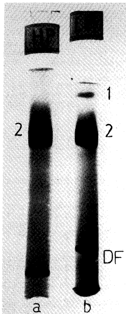
Fig.1 -- Activity staining of polyacrylamide gels for malate dehydrogenase from extracts of N. crassa grown under: a) High phosphate condition b) Low phosphate condition. DF indicates Dye Front
