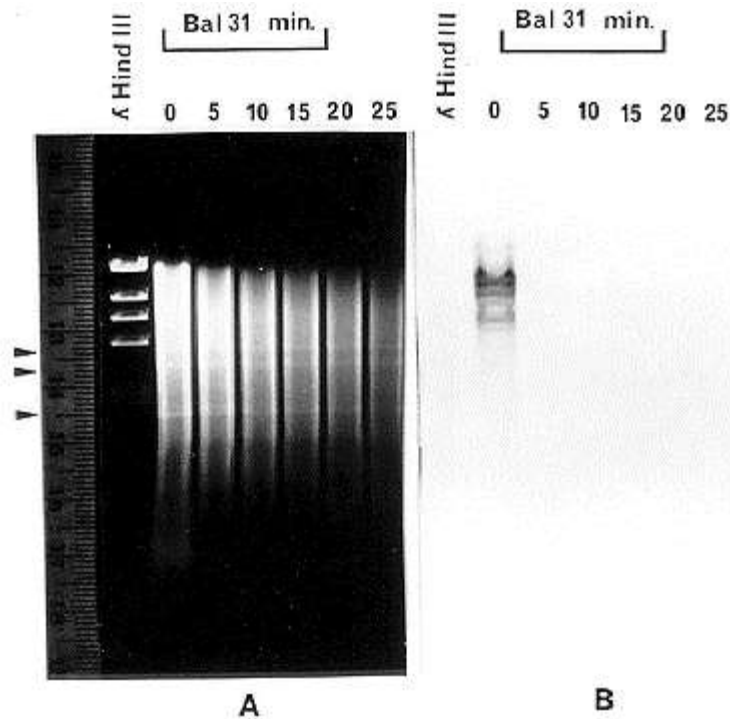
Figure 1: Bal31 digested F. oxysporum DNA probed with putative telomere sequences. Panel A. A 0.7% agarose gel containing DNA digested with Bal31 for 0, 5, 10, 15, 20, and 25 minutes. Arrow heads point to DNA bands representing interior DNA fragments. Panel B. Blot of gel in panel A, probed with ^{32}\text{P} labeled DNA fragment containing 20 telomere repeat units.
