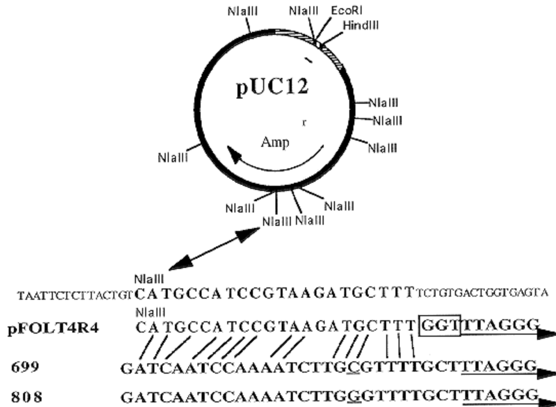
Figure 2: Comparison of sequences from: the in vivo modification site of pUC12; the DNA adjacent to the telomere repeats of the fungal-modified, autonomously replicating plasmid, pFOLT4R4; the DNA adjacent to the telomere repeats of F. oxysporum strain PHW699 (699); and the DNA adjacent to the telomere repeats of F. oxysporum strain PHW808 (808). Arrows underline the beginning of the telomere repeat units which are repeated from three to eighteen times in the different clones. The box highlights three base pairs in pFOLT4R4 which are not part of the telomere repeats and are not part of the pUC12 sequences. The underlined bases in 699 and 808 represent the single base difference between these strain's sequences. The lines between the plasmids (top two sequences) and the telomeres of F. oxysporum (third and fourth sequence) show one possible sequence similarity.
