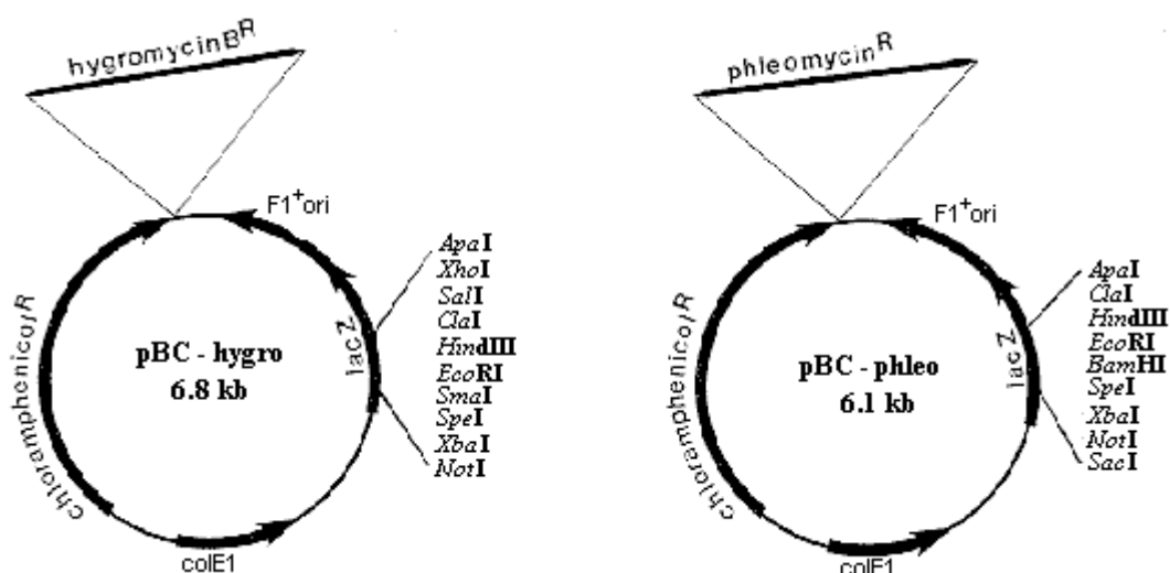
Figure 1. Two vectors for transformation of filamentous fungi. Left: pBC-Hygro. Right: pBC-phleo. For details, see text.
