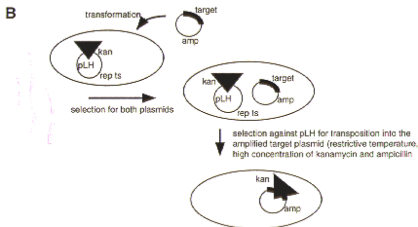
Figure 1. A. Construction of pLH1 and pLH3. pLH1: The 1.55 kb argB gene was amplified with artificial Xho I overhangs and ligated to Sal I digested pFTS. pLH3: A 1.4 kb Sal I fragment containing the hph gene was ligated to Sal I digested pFTS. B. Transposon mutagenesis using pLH1 and pLH3. Competent E. coli cells containing pLH1 or pLH3 are transformed with the plasmid containing a gene to be disrupted. Transformants containing the pLH plasmid and the target plasmid are selected on medium containing ampicillin (selection for target plasmid) and kanamycin (selection for tn5seq1). The temperature and antibiotic concentration are raised to counterselect the pLH plasmid and promote transposition as well as the amplification of the target plasmid. Plasmids that are both kanamycin and ampicillin resistant are characterized and the exact site for tn5seq1 integration determined by restriction analysis (and/or sequencing).
