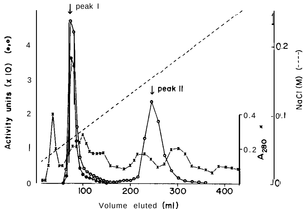
Figure 1. DEAE-cellulose chromatography of a resuspended 50-to-75% AS fraction from cellobiose-grown mycelia. The sample applied contained 101 units of \beta -galactosidase activity and 135 units of \beta -glucosidase activity. (●) \beta -galactosidase activity; (○) \beta -glucosidase activity; (x) absorbance at 280 nm; (---) NaCl concentration.
