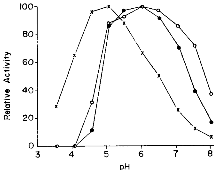
Figure 2. Effect of pH on DEAE-cellulose peak-I \beta -galactosidase activity (•), peak-I \beta -glucosidase activity (o), and peak-II \beta -glucosidase activity (x). The number of units used were: peak-I \beta -galactosidase, 1.30; peak-I \beta -glucosidase, 1.30; and peak-II \beta -glucosidase, 1.84. Activities were measured at pH optima.
