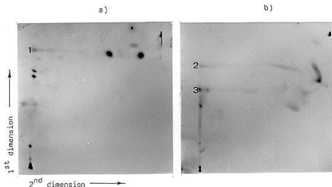
Figure 2. Autoradiography of the two-dimensional thin layer chromatography of the chloroform-extractable metabolites of the [ ^{14}\text{C} ]acetate-labelled mutant (a) and the wild-type strain (b). Extraction of CA and the solvent system of each dimension are described in the text. 1,2,3 = separable spots by using the second solvent system.
