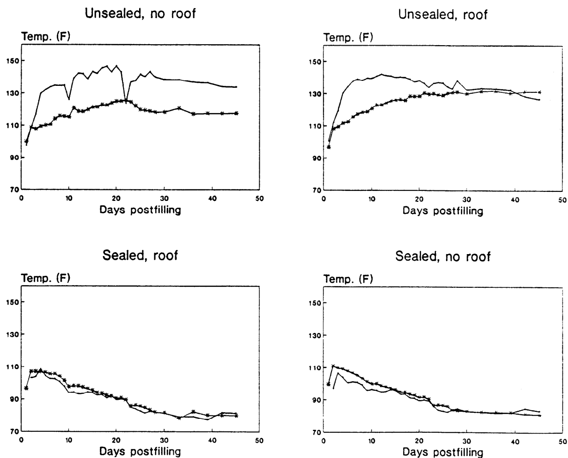
Figure 2. Effect of Sealing Treatment on the Temperature of the Alfalfa Silages during the First 6 Weeks of Storage in the Farm-scale Silos (depth below the initial surface: —□— = 5 inches and -+- 20 inches)
