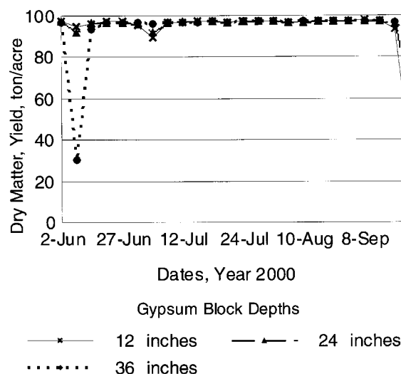
Fig. 8. Gypsum block readings at midpoint drip tape at 40 inches spacing.
