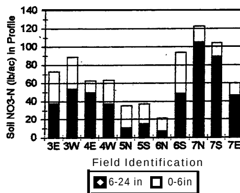
Figure 10. Soil Nitrate (lb/acre) Available from Crop Utilization from Fields Receiving Dairy Manure in South Central Kansas.
