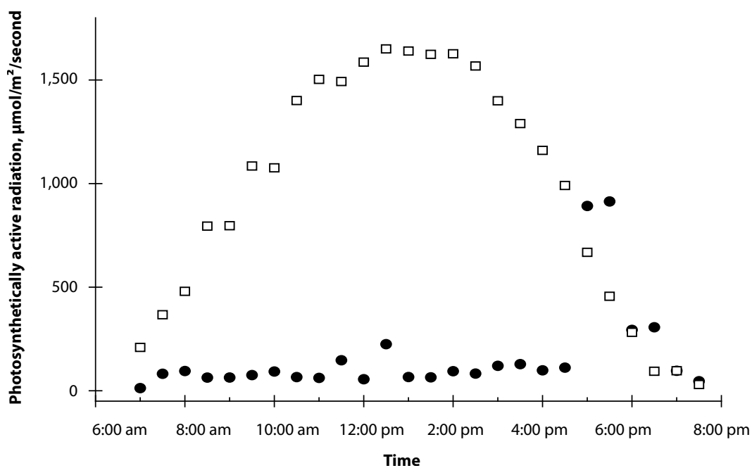
Figure 2. Mean photosynthetically active radiation under tree shade and in full sun on August 10 and 11, 2010.
