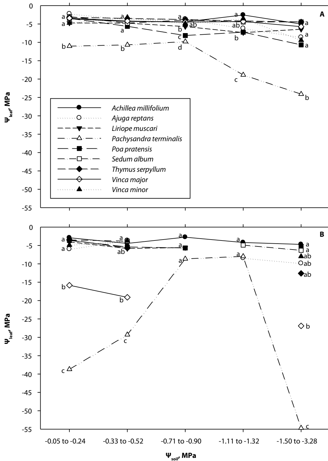
Figure 6. Changes in leaf water potential ( \Psi_{\text{leaf}} ) among species as the soils dried (i.e., \Psi_{\text{soil}} became more negative) during the spring/summer (A) and the fall (B) drydown. Means followed by the same letter within each \Psi_{\text{soil}} range are not significantly different ( P = 0.05 ).
