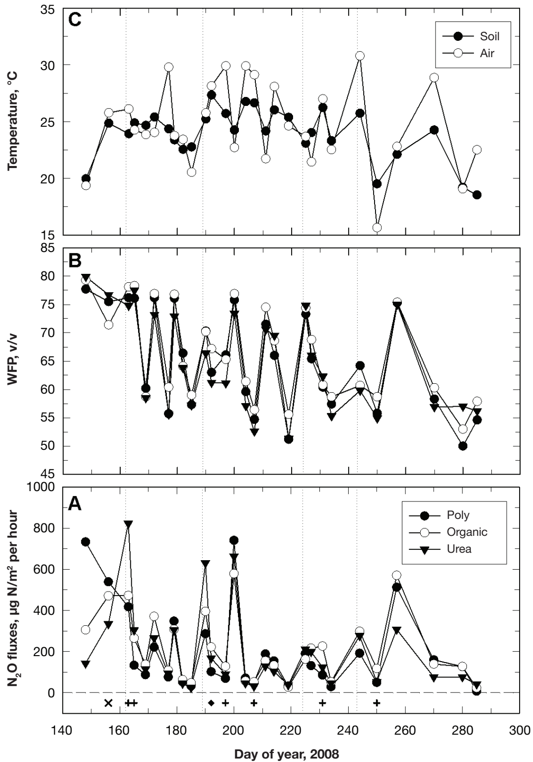
Figure 2. (A) Fluxes of N_2O -N from plots fertilized with polymer-coated urea (poly), organic nitrogen, and urea; (B) water-filled porosity (WFP) in the 0- to 6-in. profile; (C) average soil temperature at 2 in. among treatments and air temperature at 6.5 ft at sampling.
