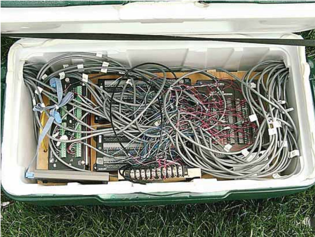
Figure 4. Data acquisition system used to log soil moisture data. The system included a datalogger and three multiplexors and was capable of controlling 32 dual-probe heat-capacity sensors.
