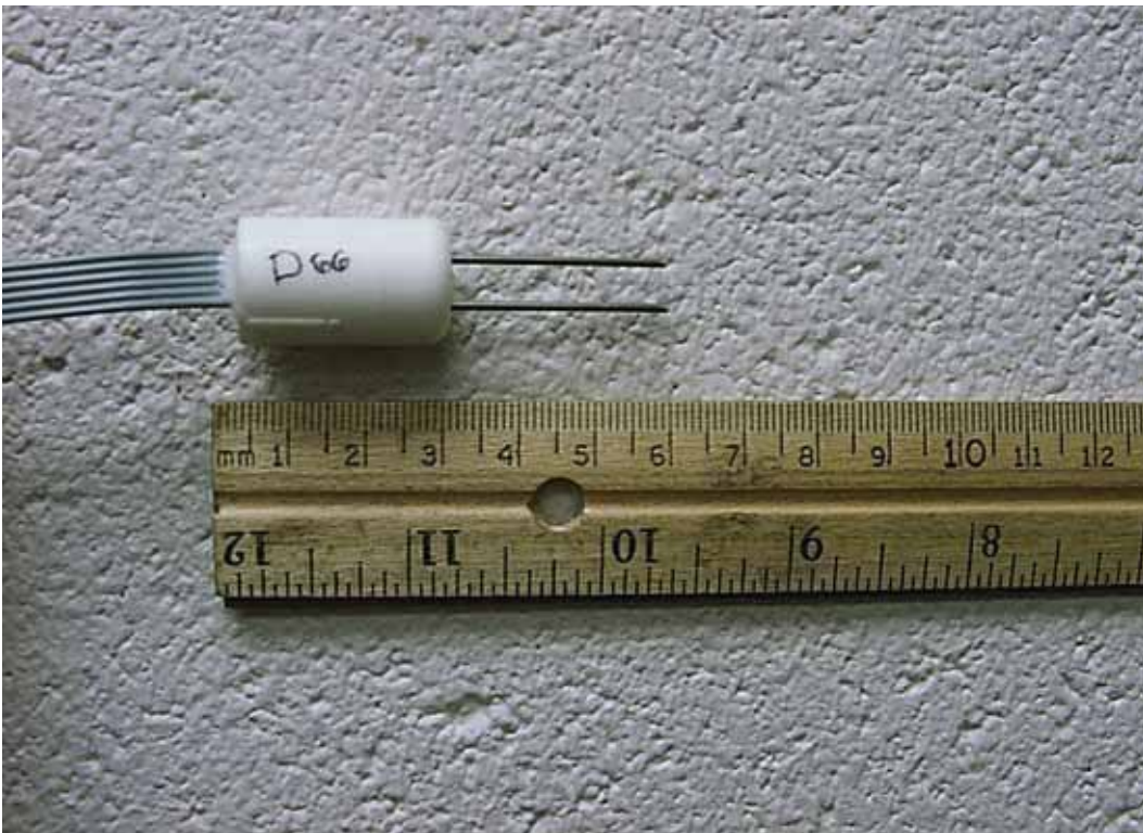
Figure 2. A dual-probe heat-capacity sensor built at K-State to measure soil moisture at specific depths.
