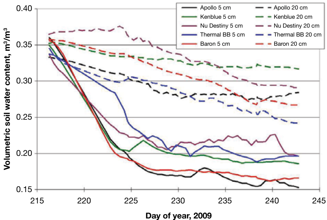
Figure 6. Measurements of volumetric soil water content at 2 in. (5 cm) and 8 in. (20 cm) during the 26-day drydown among four Kentucky bluegrasses and a hybrid bluegrass (Thermal Blue Blaze).
