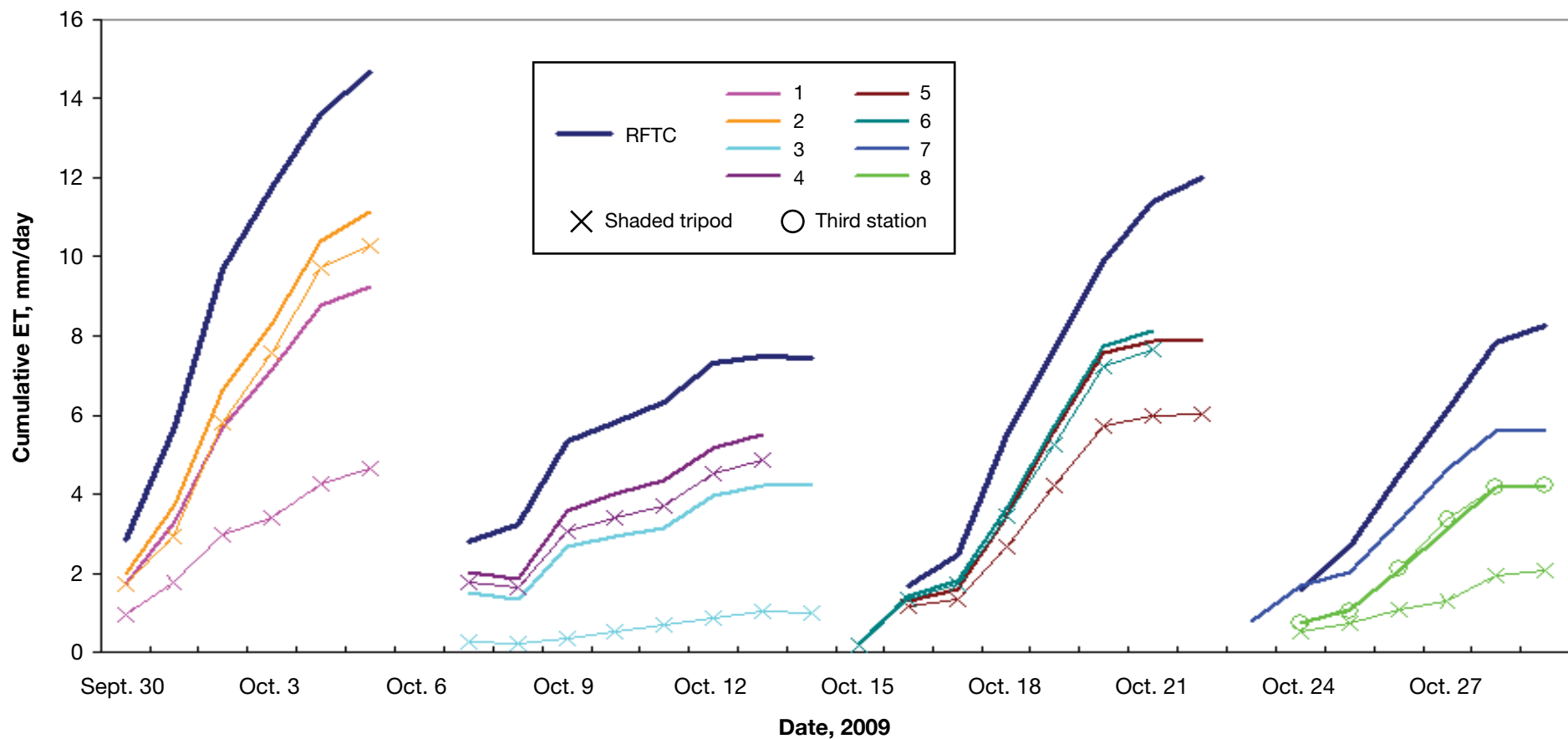
Figure 5. Cumulative reference crop evapotranspiration (ET 0 ) from all lawn-deployed tripods compared with that from the tripod at the Rocky Ford Turfgrass Research Center.
