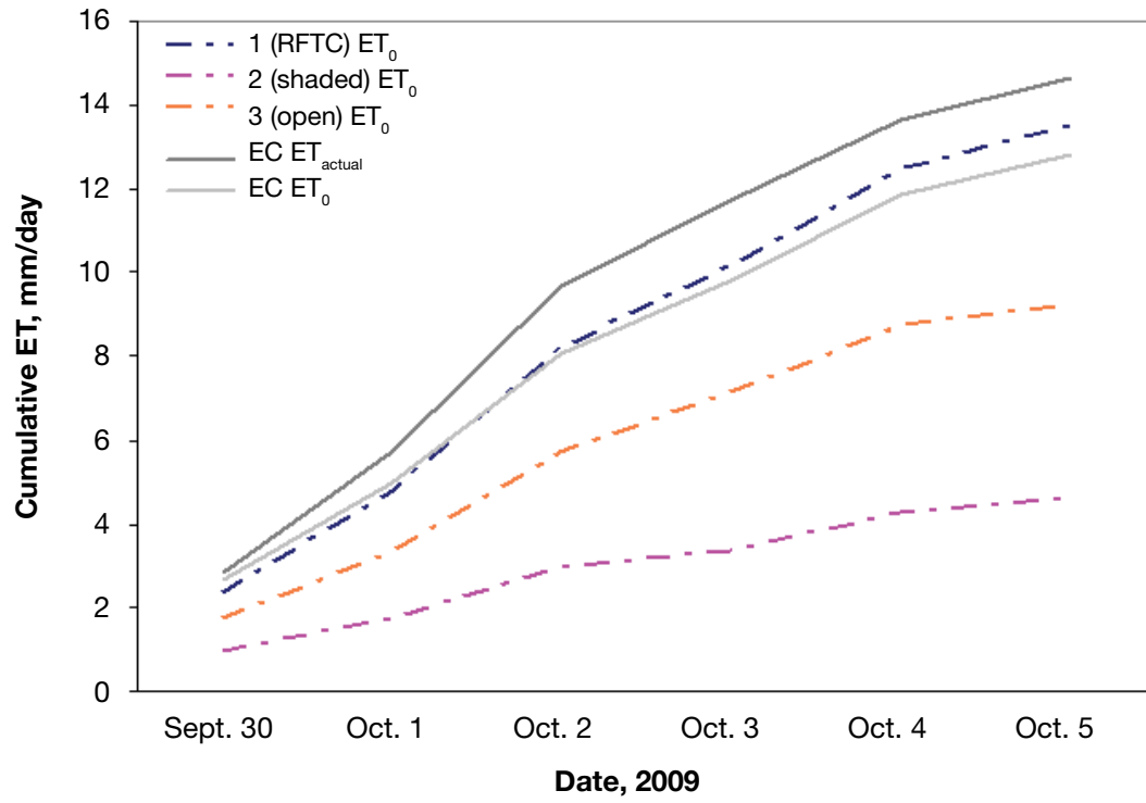
Figure 4. Cumulative reference crop evapotranspiration ( ET_0 ) reported by three tripods during deployment on one property and cumulative ET_0 and actual evapotranspiration ( ET_{actual} ) as measured at the eddy covariance (EC) site.
