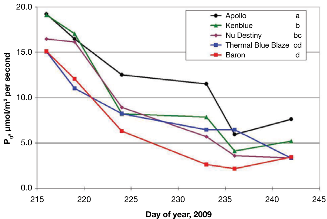
Figure 5. Estimates of gross photosynthesis ( P_g ) during a 26-day drydown for four Kentucky bluegrasses and a hybrid bluegrass (Thermal Blue Blaze). In legend, cultivar names followed by the same letter were not significantly different in terms of cumulative P_g during the drydown.
