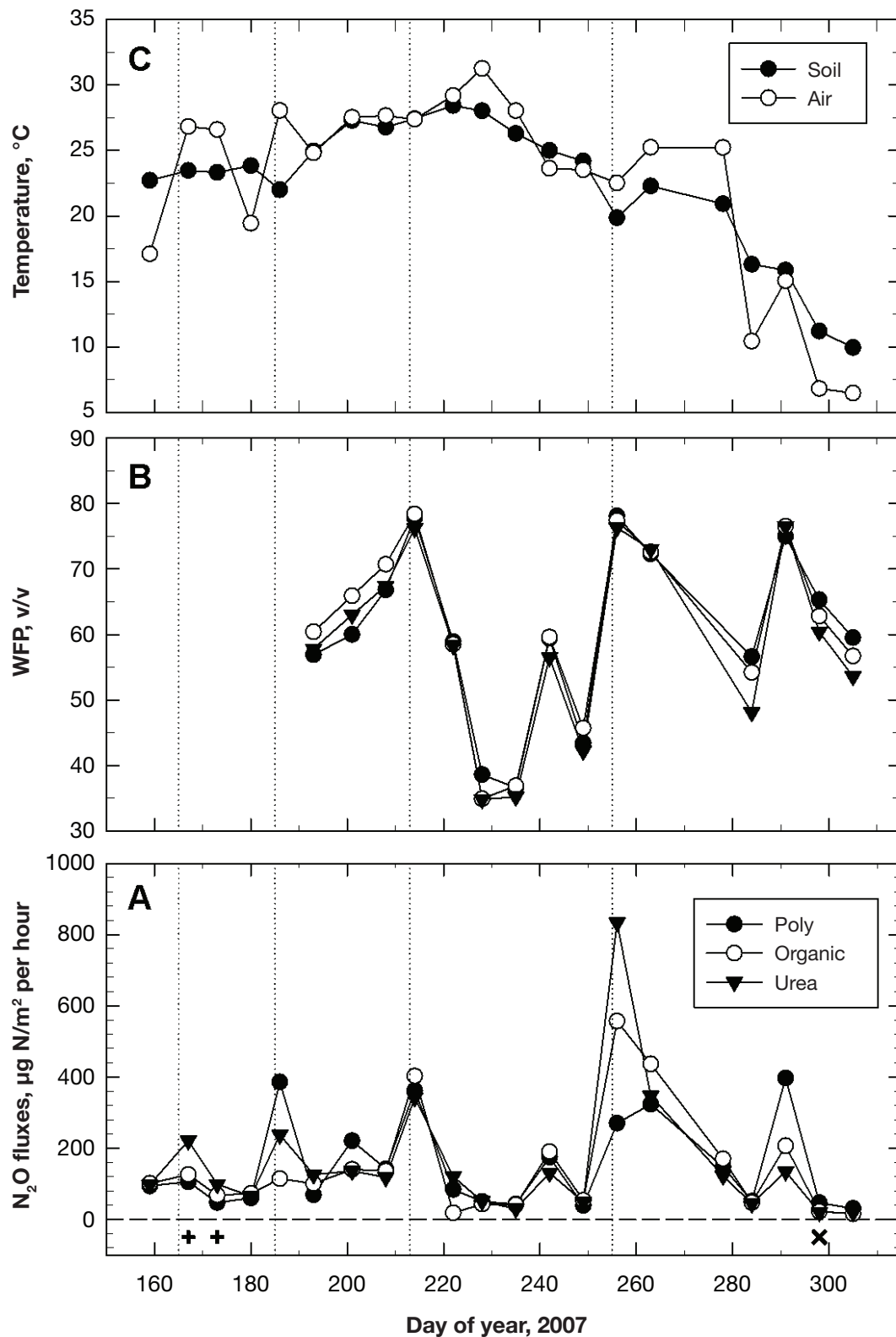
Figure 1. (A) Fluxes of N_2O -N from plots fertilized with polymer-coated urea (poly), organic nitrogen, and urea; (B) water-filled porosity (WFP) in the 0- to 6-in. profile; (C) average soil temperature at 2 in. among treatments and air temperature at 6.5 ft during sampling periods.
