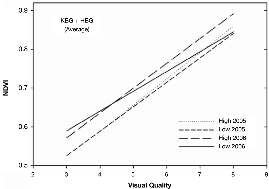
Figure 3. Relationships between normalized difference vegetation index (NDVI) and visual quality.
