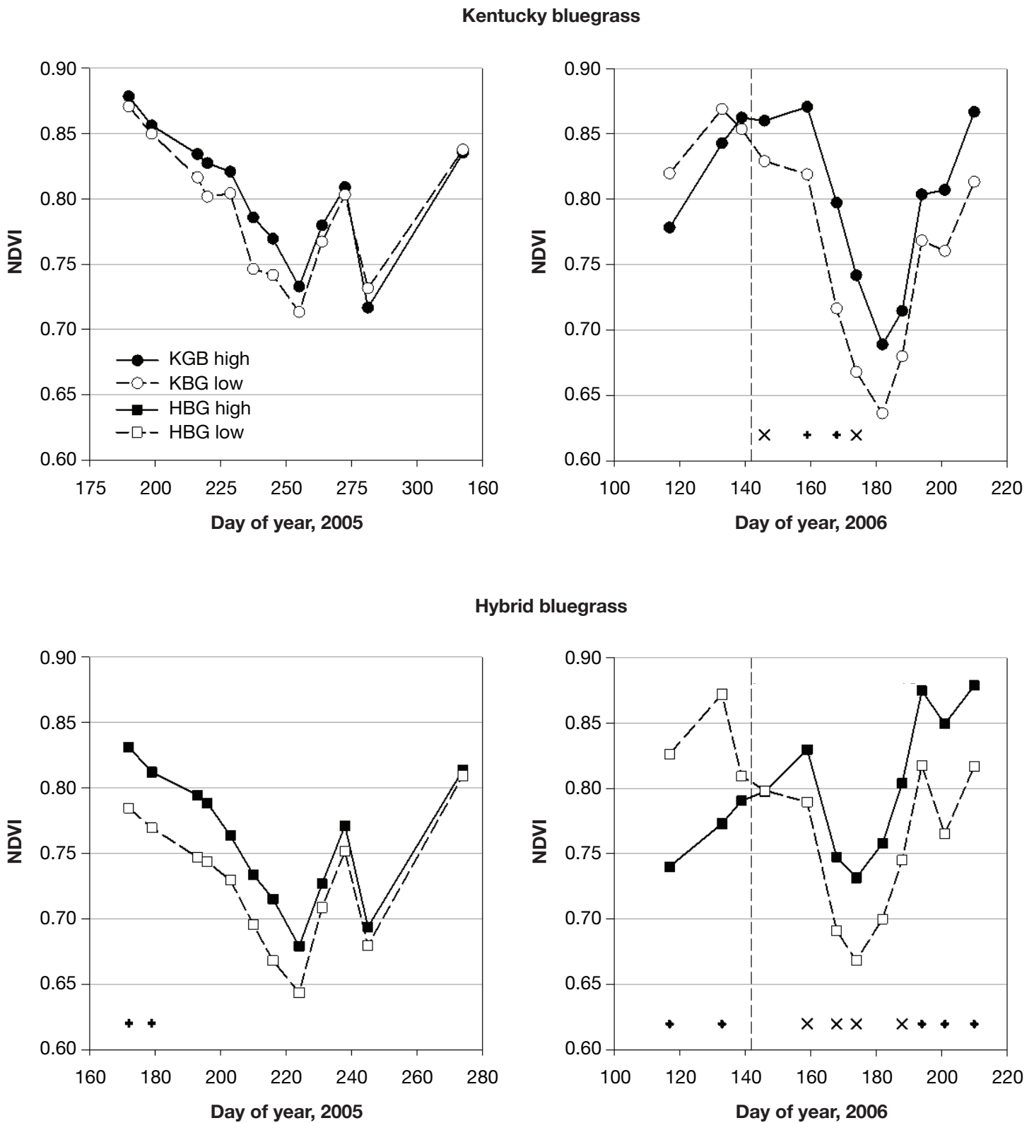
Figure 1. Normalized difference vegetation index (NDVI) in high-mown (3 in.) and low-mown (1.5 in.) plots of Kentucky bluegrass (Apollo) and a hybrid bluegrass (Thermal Blue) during 2005 and 2006.
