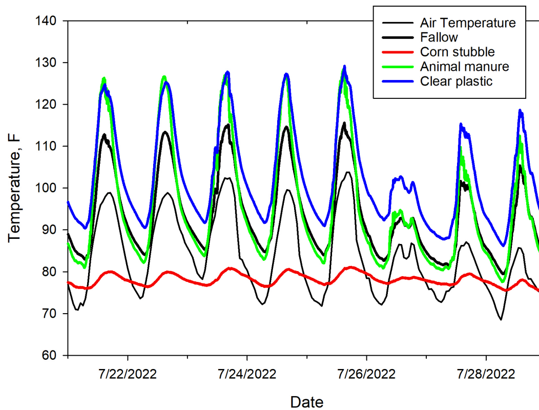
Figure 1. Temperatures (°F) at 2-in. soil depth in the different treatments.
