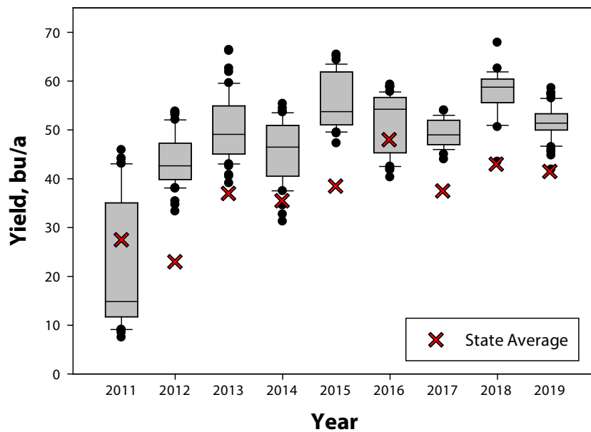
Figure 5. Soybeans from (A) MG3-4 and (B) MG4-5 from variety trials grown at Columbus, Erie, and Parsons, KS, from 2011 through 2019. For comparison, average reported yields from Kansas are highlighted as a red X.
