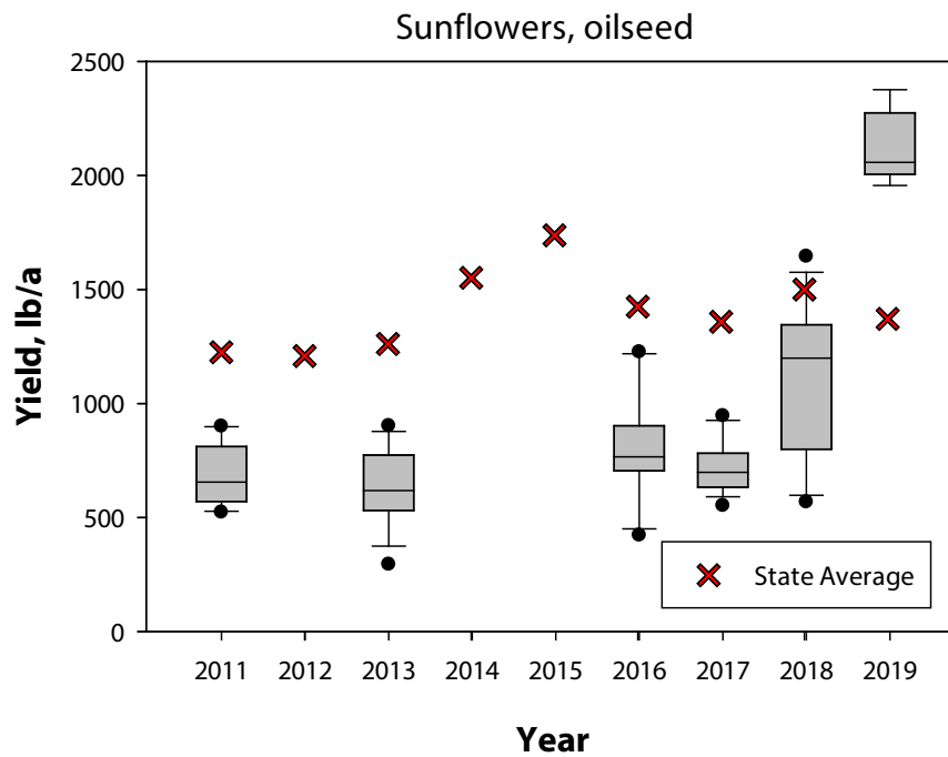
Figure 7. Oilseed sunflowers from variety trials grown at Parsons, KS, from 2011 through 2019. Yield data were not available from the variety plots in 2012, 2014, or 2015. For comparison, average reported Kansas state yields are highlighted as a red X.
