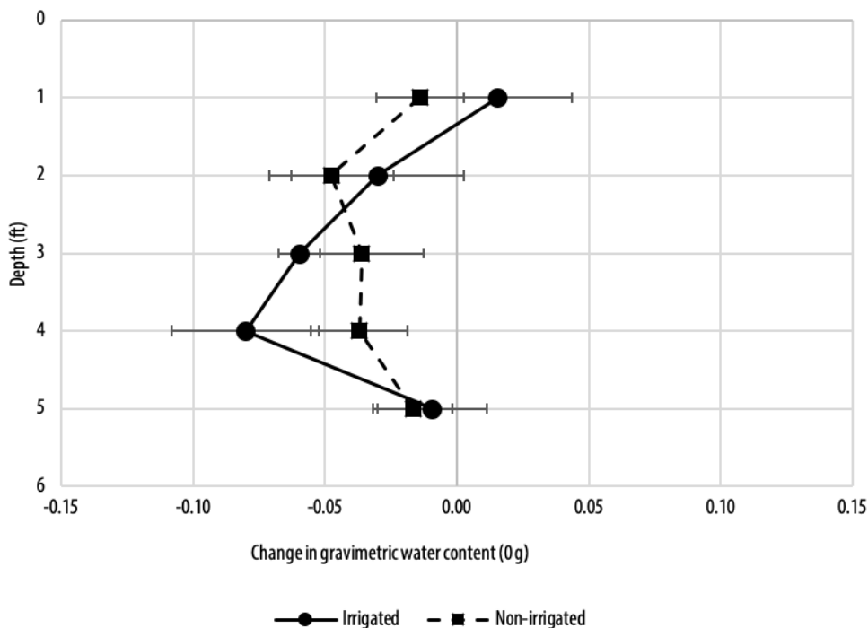
Fig 5. Soil moisture change in irrigated and unirrigated plots of hemp (SS Beta), July - September 2019.
