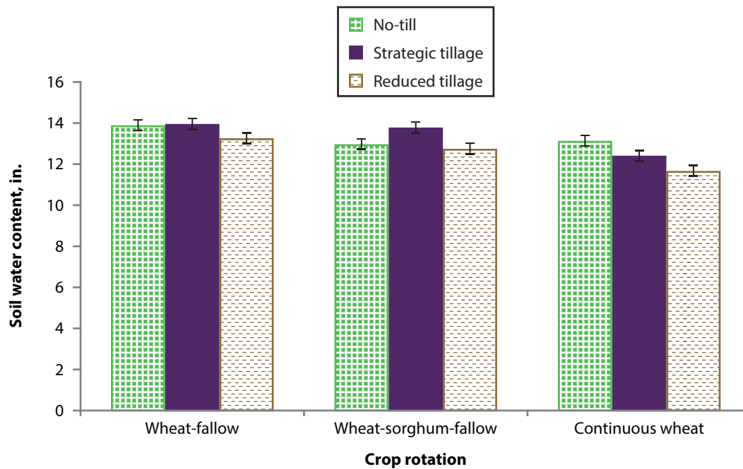
Figure 1. Soil water content at winter wheat planting as affected tillage in each crop rotation system. Data are averaged across 2 year and three replications (n = 6).
