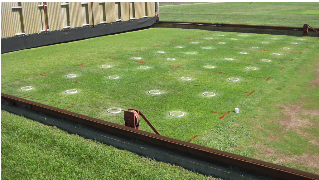
Figure 1. Automated rainout shelter that is activated by 0.01 inch of rain.
