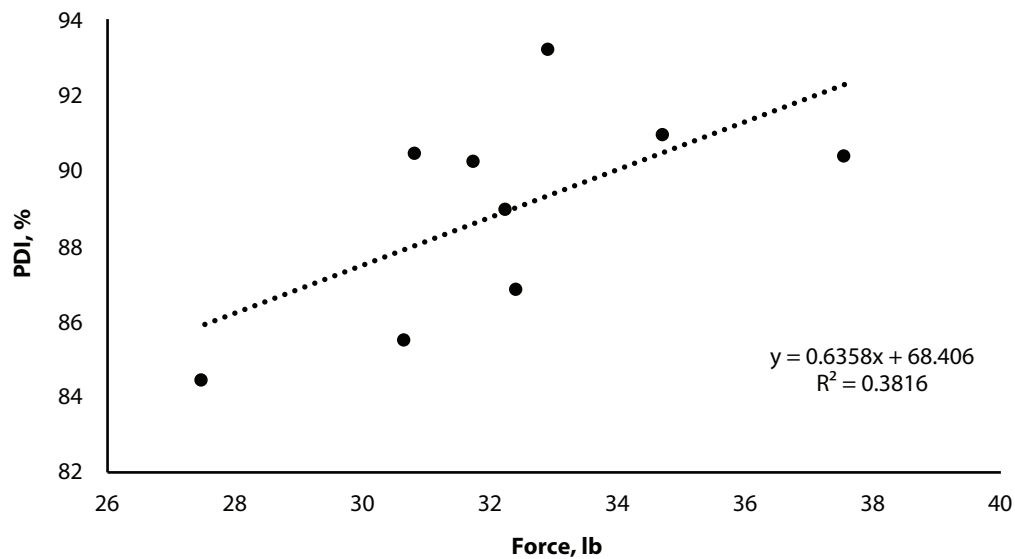
Figure 1. The relationship of pellet hardness (Force) and pellet durability index (PDI).
