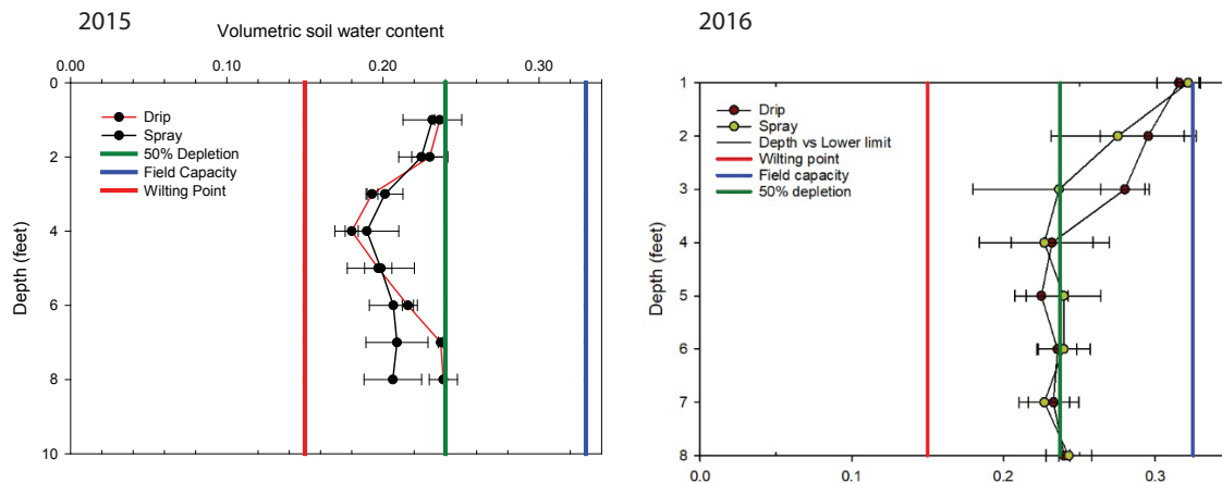
Figure 13. End-of-season soil water measurements under mobile drip irrigation and spray nozzles for well capacity of 600 gpm during the 2015 and 2016 growing seasons at the Kansas State University Southwest Research-Extension Center, near Garden City, KS.
