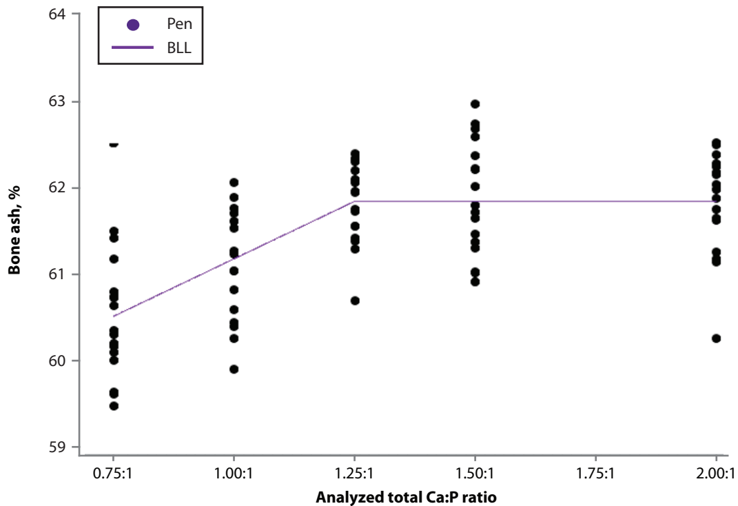
Figure 5. Fitted broken-line linear (BLL) regression model on percentage bone ash as a function of increasing analyzed calcium:phosphorus ratio in growing-finishing pigs fed diets containing 1,000 phytase units. The BLL model estimated the maximum mean percentage bone ash at 1.25 analyzed Ca:P ratio (95% CI: [1.10:1, 1.40:1]). The estimated regression equation was bone ash, % = 61.83 - 2.65158 \times (\text{Ca:P}) if analyzed Ca:P ratio < 1.25:1. If analyzed Ca:P \geq 1.25:1, then bone ash, % = 61.83.
