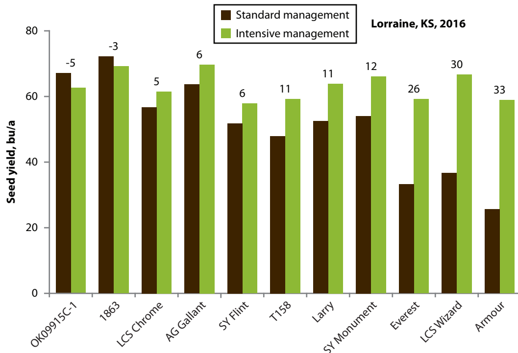
Figure 2. Wheat grain yield as affected by variety and management strategy in Lorraine and Ellsworth, KS, during the 2015-2016 growing season. Varieties with greater susceptibility to stripe rust, such as Everest, LCS Wizard, and Armour, also show the greatest yield gap.
