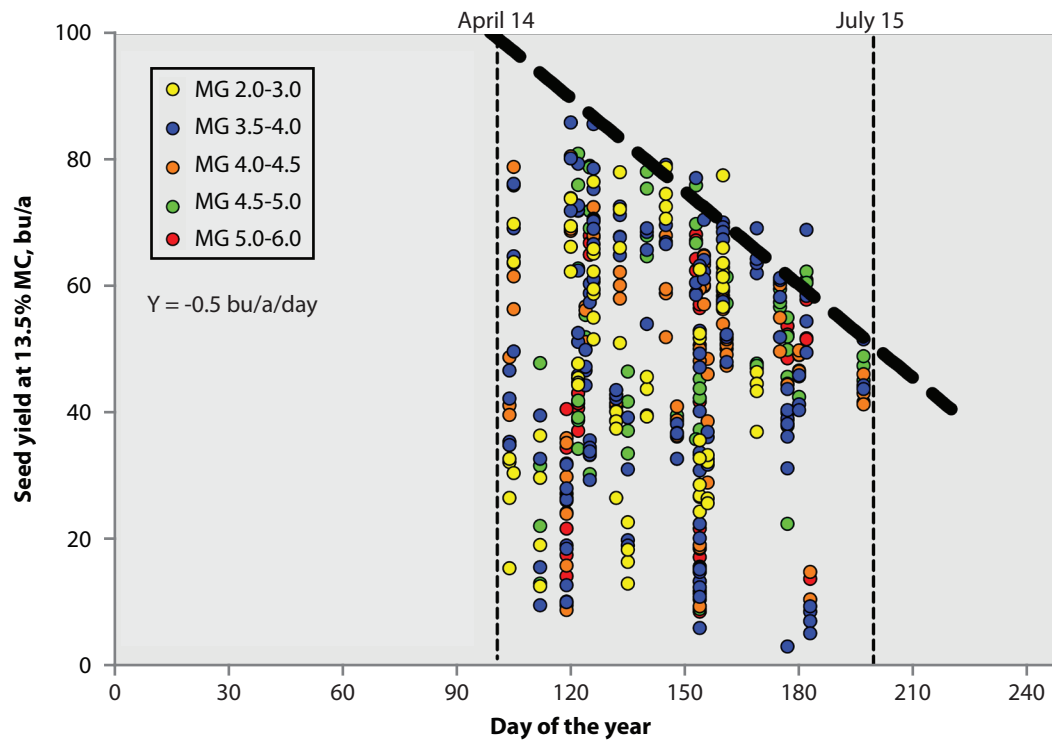
Figure 7. Soybean yield (bushels per acre) for all soybean studies with different planting dates (early, mid, and late) and maturity groups (MG) at 13 sites across Kansas during the 2014, 2015, and 2016 growing seasons. A frontier line was determined for the points with high yield. MC = moisture content.
