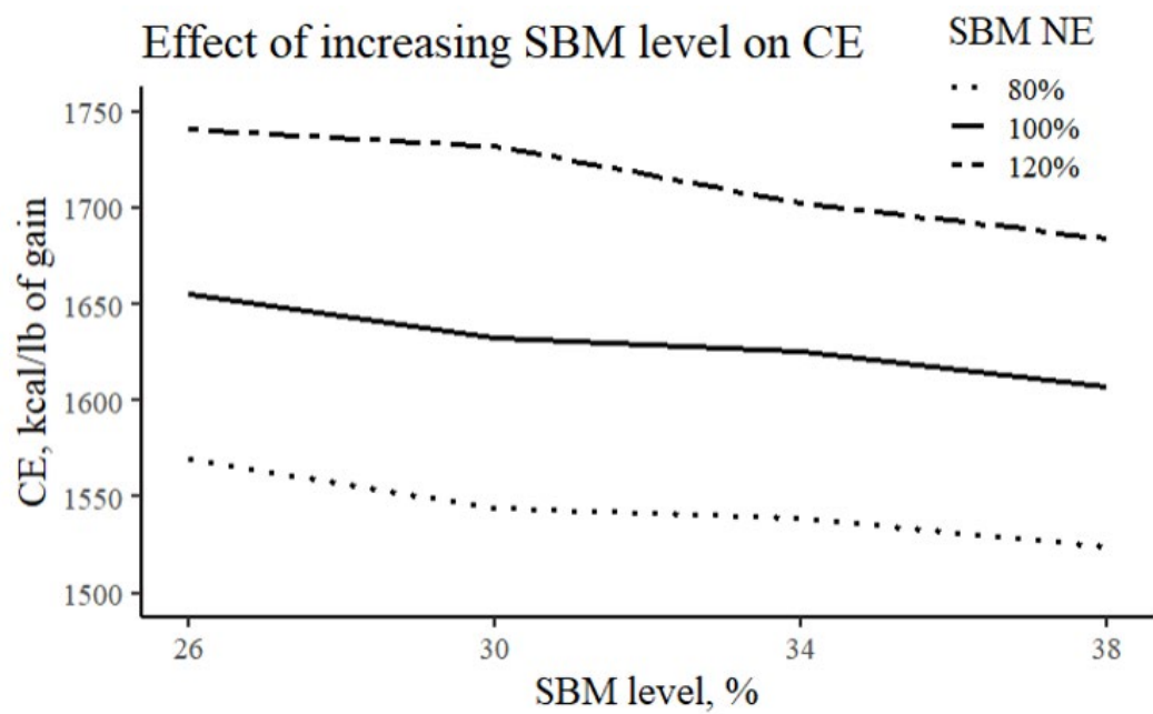
Figure 1. Effect of increasing soybean meal (SBM) level on caloric efficiency (CE) when SBM NE is estimated at 80, 100, or 120% of corn NE in diet formulation. For 80% SBM NE, slope = -3.55. 100% SBM NE, slope = -3.81. 120% SBM NE, slope = -4.98. Increasing SBM level within 80% SBM NE: linear, P < 0.001 ; quadratic, P = 0.508 . Increasing SBM level within 100% SBM NE: linear, P < 0.001 ; quadratic, P = 0.999 . Increasing SBM level within 120% SBM NE: linear, P < 0.001 ; quadratic, P = 0.610 .
