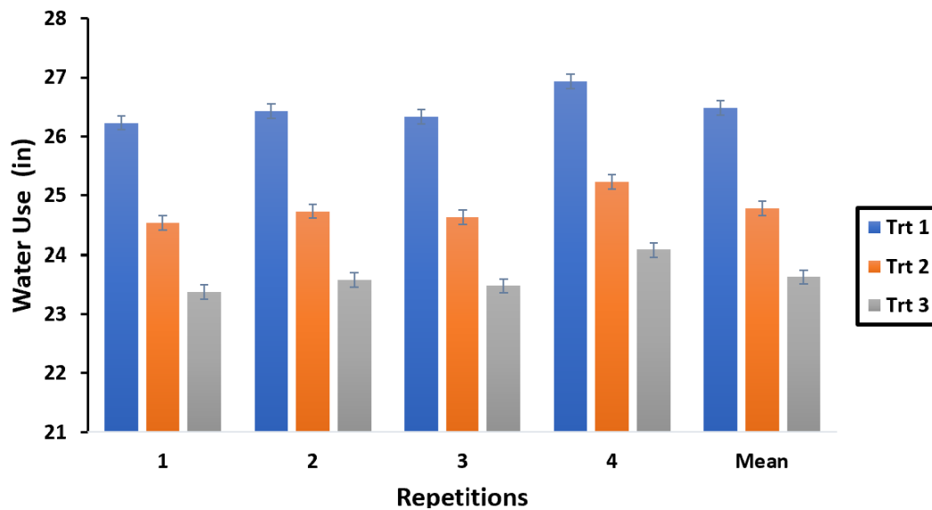
Figure 3. Water use (inches) for the three irrigation treatments designed to match 100%, 85%, and 75% of well-watered corn ET minus rain.
