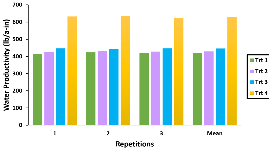
Figure 2. Water productivity (lb/a-inch) with different irrigation treatments.
