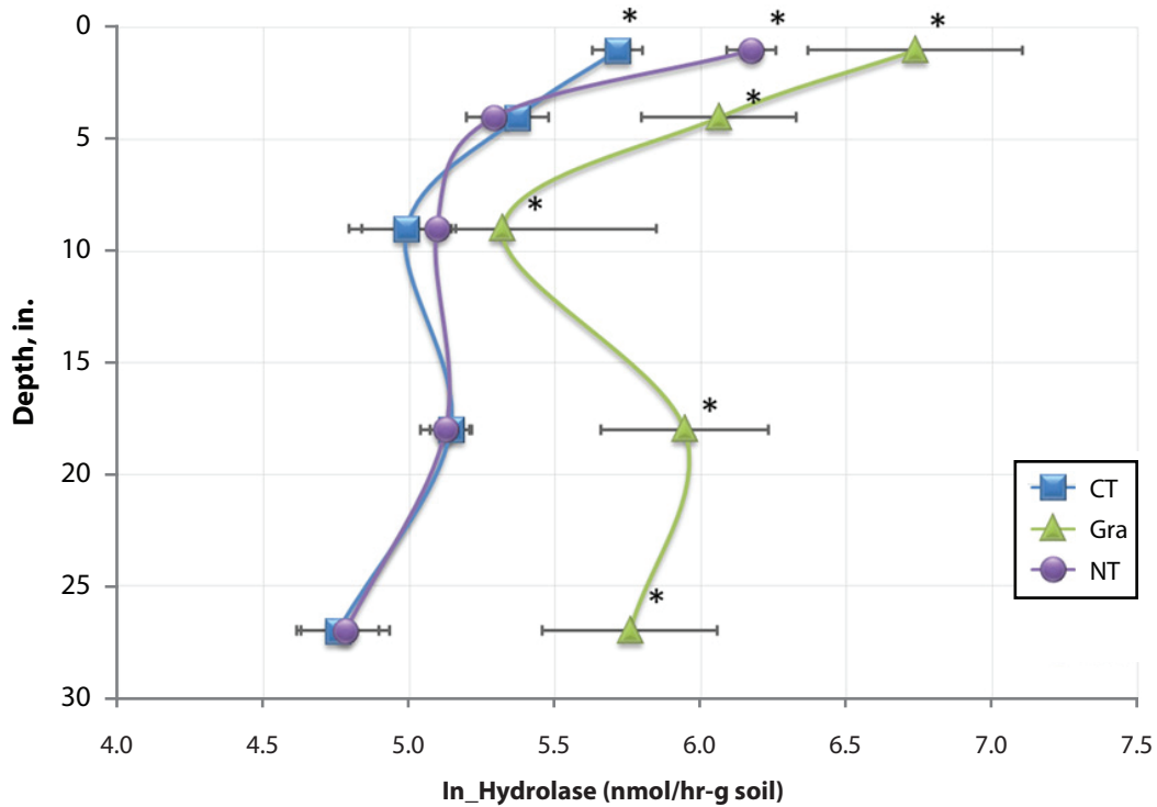
Figure 1. Change in soil hydrolase activity with depth measured as the amount of hydrolase activity (nmol) per hour for a standard weight of soil for three different management systems, Conventional Till crop production (CT), No-Till crop production (NT) and Grassland (Gra). *Significant difference at 95% confidence level.
