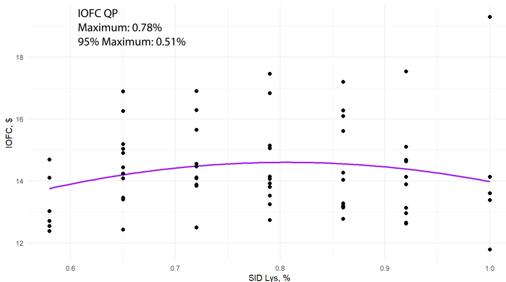
Figure 3. Estimation of SID Lys requirement to maximize IOFC at high ingredient and pig prices for 170 to 220 lb DNA finishing pigs.
