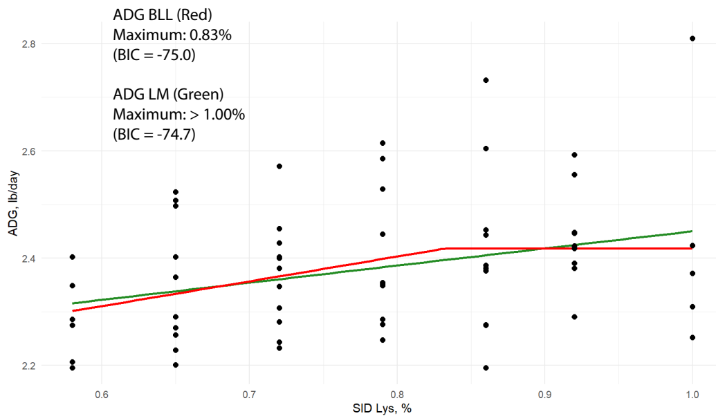
Figure 1. Estimation of SID Lys requirement to maximize ADG for 170 to 220 lb DNA finishing pigs.
