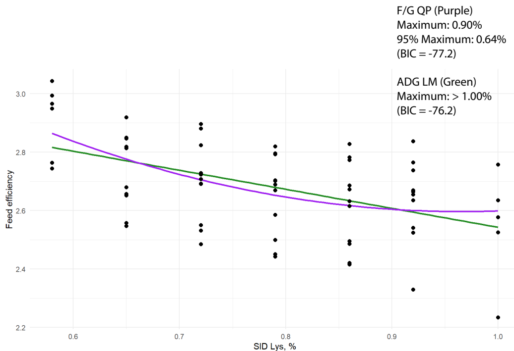
Figure 2. Estimation of SID Lys requirement to optimize F/G for 170 to 220 lb DNA finishing pigs.
