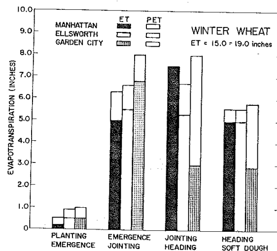
Fig. 4.—Evapotranspiration (ET) and potential evapotranspiration (PET) of winter wheat at various stages
