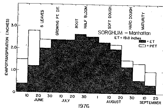
Fig. 3.—Seasonal trends in evapotranspiration (ET) and potential evapotranspiration (PET) of sorghum at Manhattan, Kansas, 1976.
