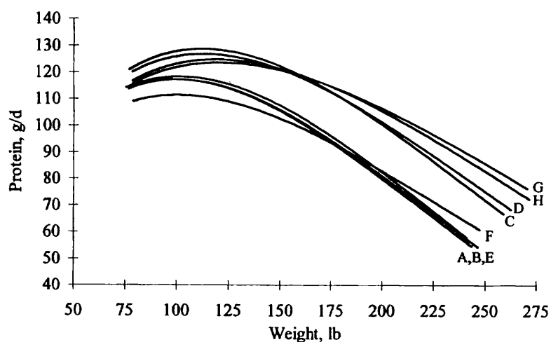
Figure 2. Modeled Daily Protein Accretion for Barrows Fed Diets with Increasing Lysine:Calorie Ratios and Two Dietary Fat Levels.
