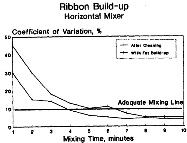
Figure 4. Effect of ribbon build-up on mixing efficiency,
