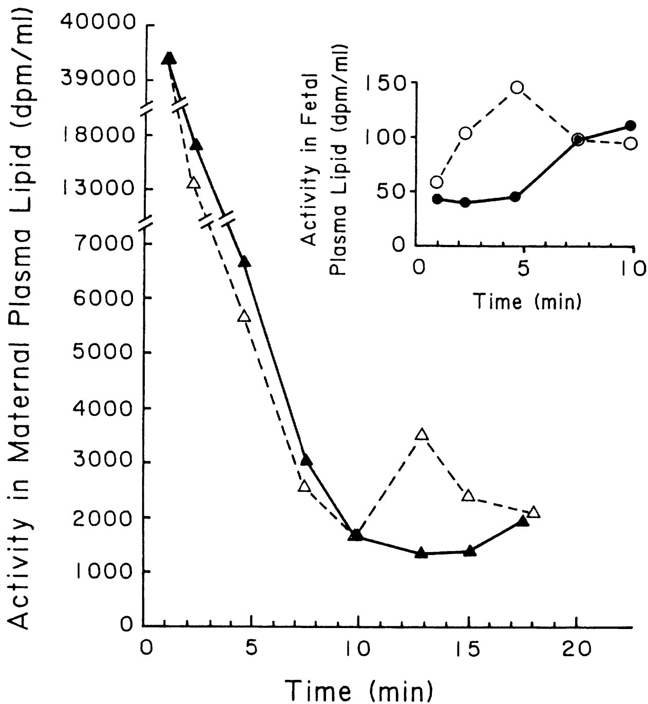
Figure 6. Radioactivity in maternal and fetal plasma lipid following maternal injection of 100 \mu Ci of [^3\text{H}] palmitic acid (Exp. 3). Solid circle ( ● ) represents FV; open circle ( ○ ) represents FA; solid triangle ( ▲ ) represents UV and open triangle ( △ ) represents UA.
