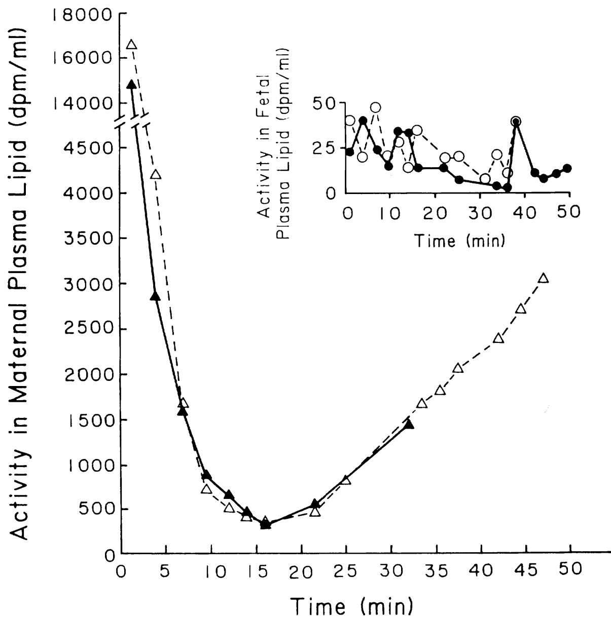
Figure 5. Radioactivity in maternal and fetal plasma lipid following maternal injection of 100 \mu Ci of [ ^3 H] palmitic acid (Exp. 2). Solid circle ( \bullet ) represents FV; open circle ( \circ ) represents FA; solid triangle ( \blacktriangle ) represents UV and open triangle ( \triangle ) represents UA.
