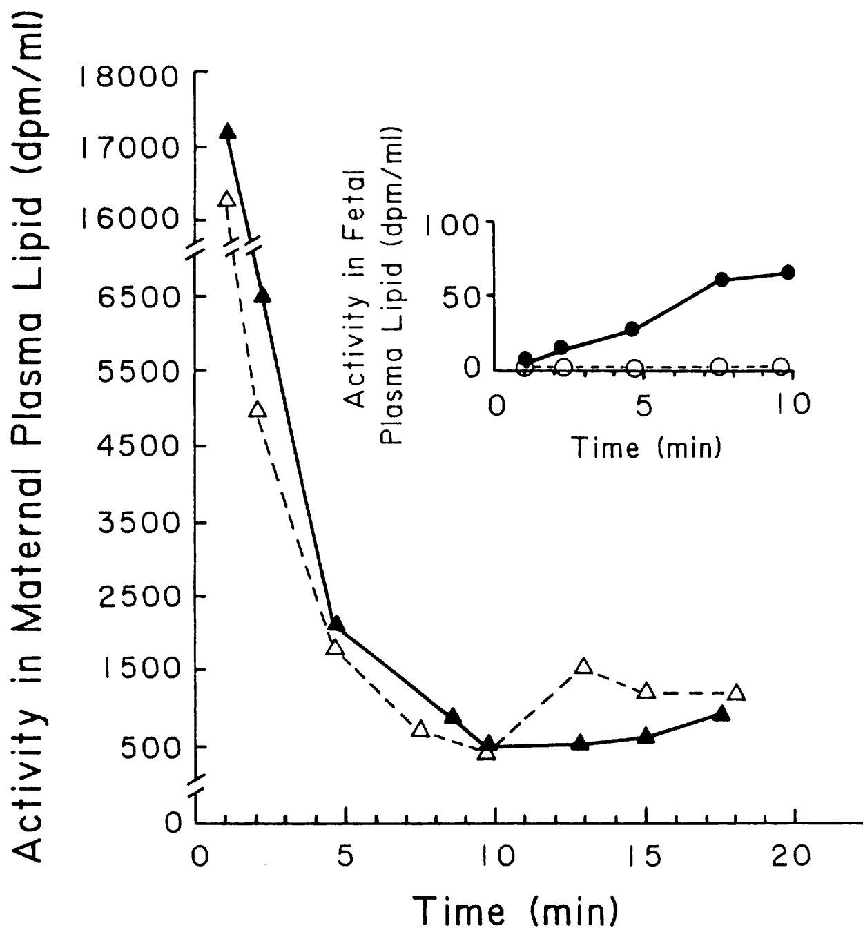
Figure 3. Radioactivity in maternal and fetal plasma lipid following maternal injection of 100 \mu\text{Ci} of [^{14}\text{C}] linoleic acid (Exp. 3). Solid circle ( \bullet ) represents FV; open circle ( \circ ) represents FA; solid triangle ( \blacktriangle ) represents UV and open triangle ( \triangle ) represents UA.
