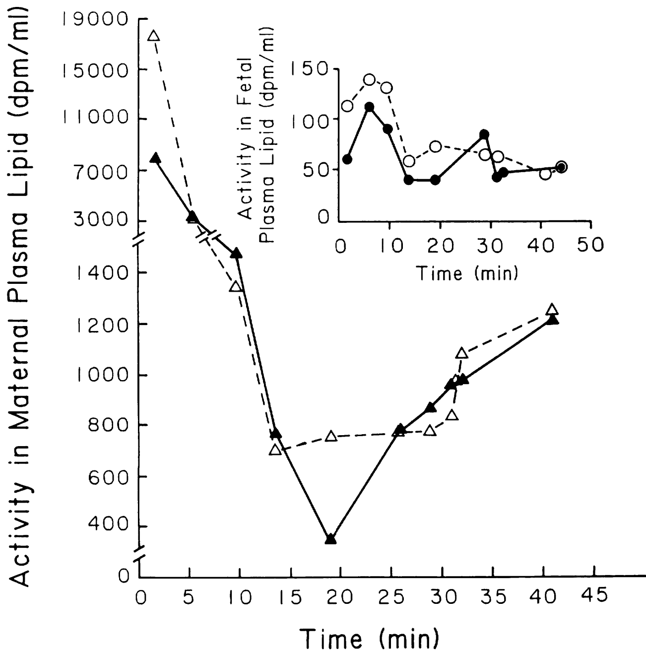
Figure 4. Radioactivity in maternal and fetal plasma lipid following maternal injection of 100 \mu Ci of [ ^3 H] palmitic acid (Exp. 1). Solid circle ( ● ) represents FV; open circle ( ○ ) represents FA; solid triangle ( ▲ ) represents UV and open triangle ( △ ) represents UA.
