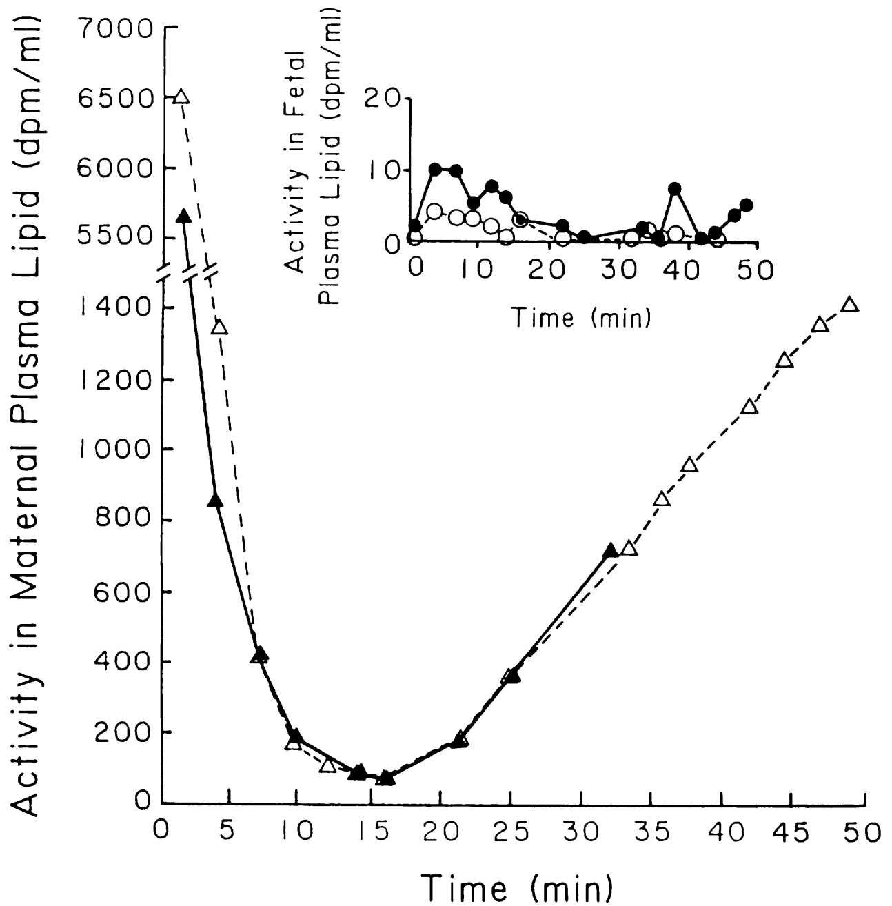
Figure 2. Radioactivity in maternal and fetal plasma lipid following maternal injection of 100 \mu\text{Ci} of [ ^{14}\text{C} ] linoleic acid (Exp. 2). Solid circle ( \bullet ) represents FV; open circle ( \circ ) represents FA; solid triangle ( \blacktriangle ) represents UV and open triangle ( \triangle ) represents UA.
