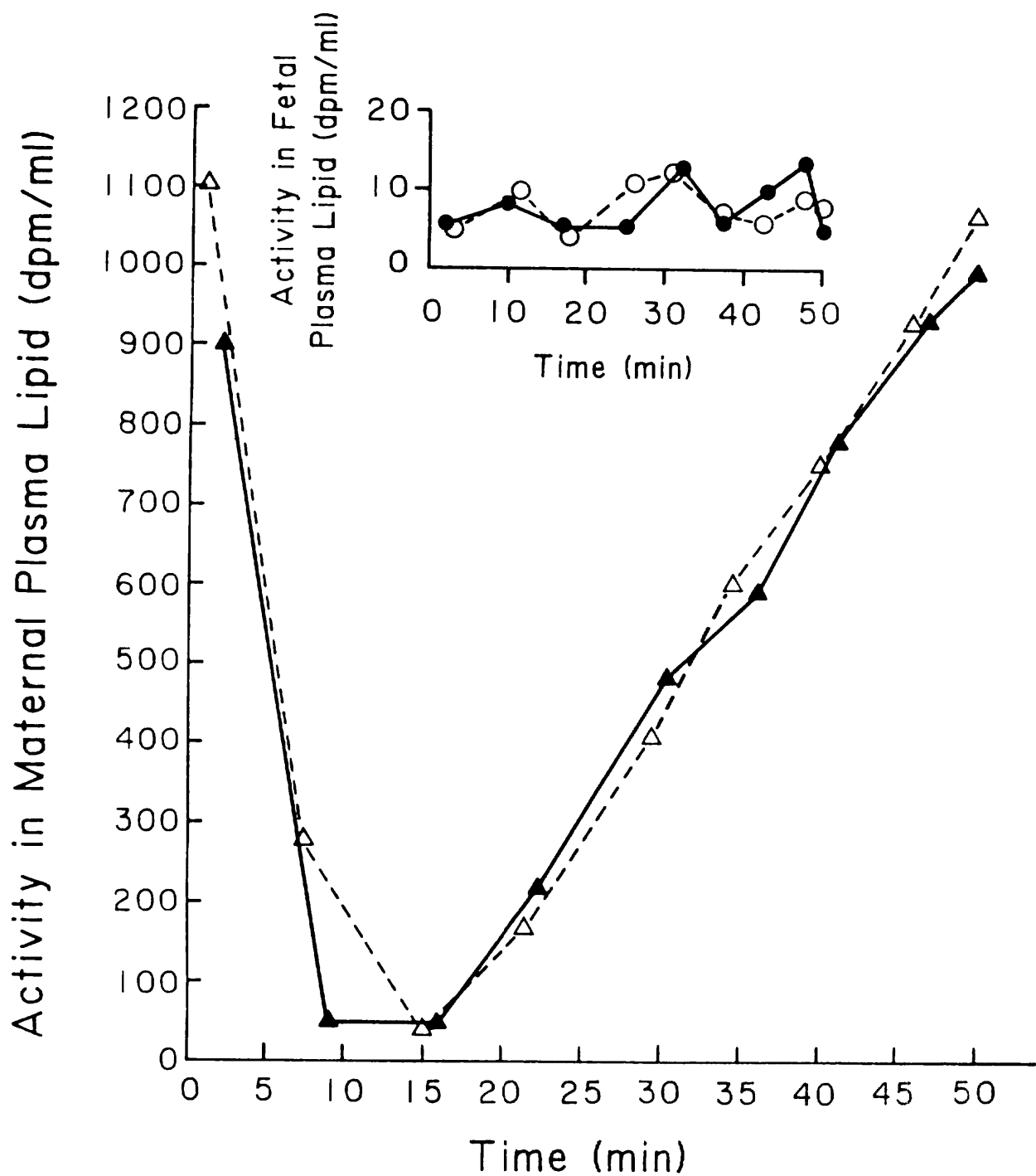
Figure 8. Radioactivity in maternal and fetal plasma lipid following maternal injection of 250 \mu Ci of [ ^{14} C] octanoic acid (Exp. 5). Solid circle ( \bullet ) represents FV; open circle ( \circ ) represents FA; solid triangle ( \blacktriangle ) represents UV and open triangle ( \triangle ) represents UA.
