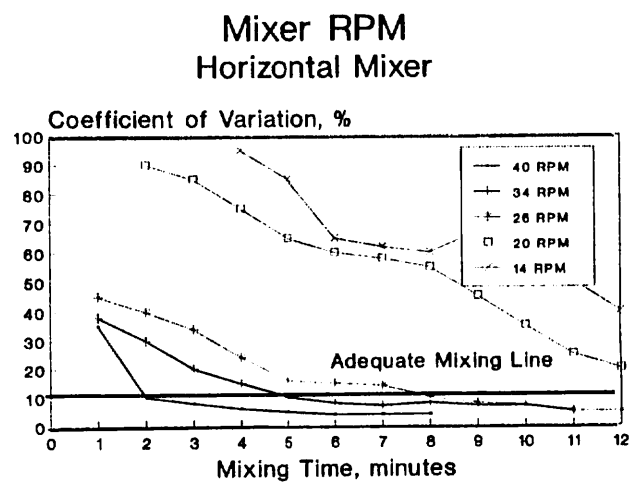
Figure 5. Effect of mixer RPM on mixing efficiency.
