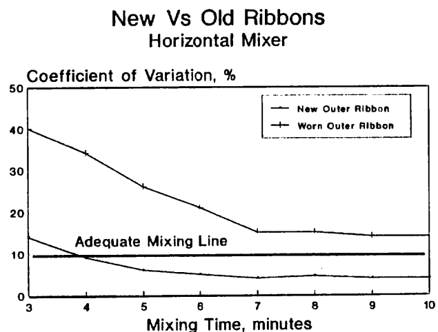
Figure 3. Effect of a wear on mixing efficiency of a single-screw mixer.
