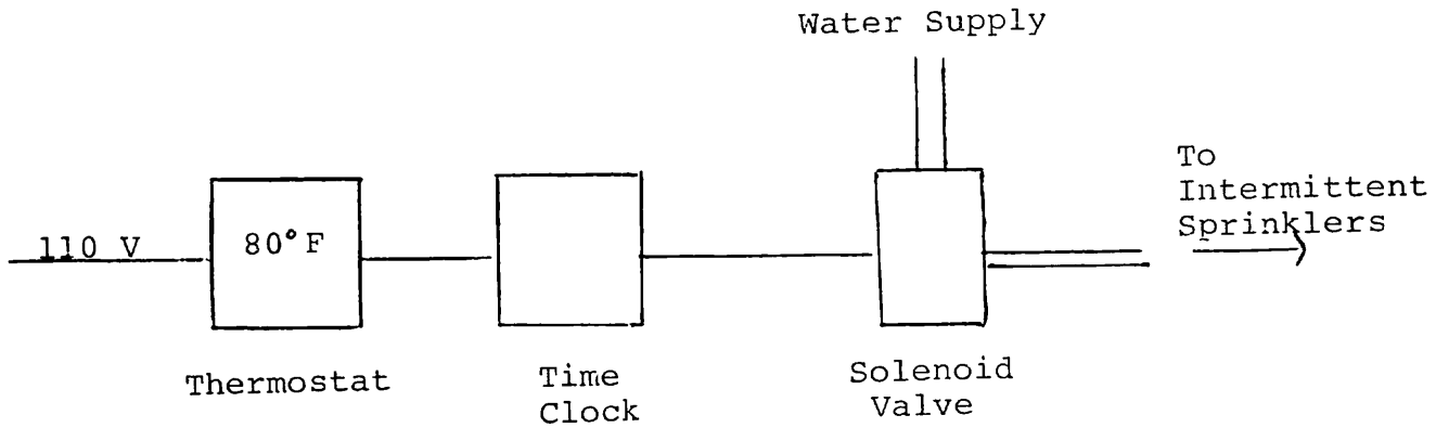
INTERMITTENT SYSTEM
