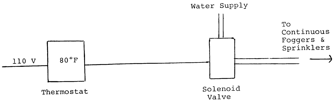
CONTINUOUS SYSTEM
