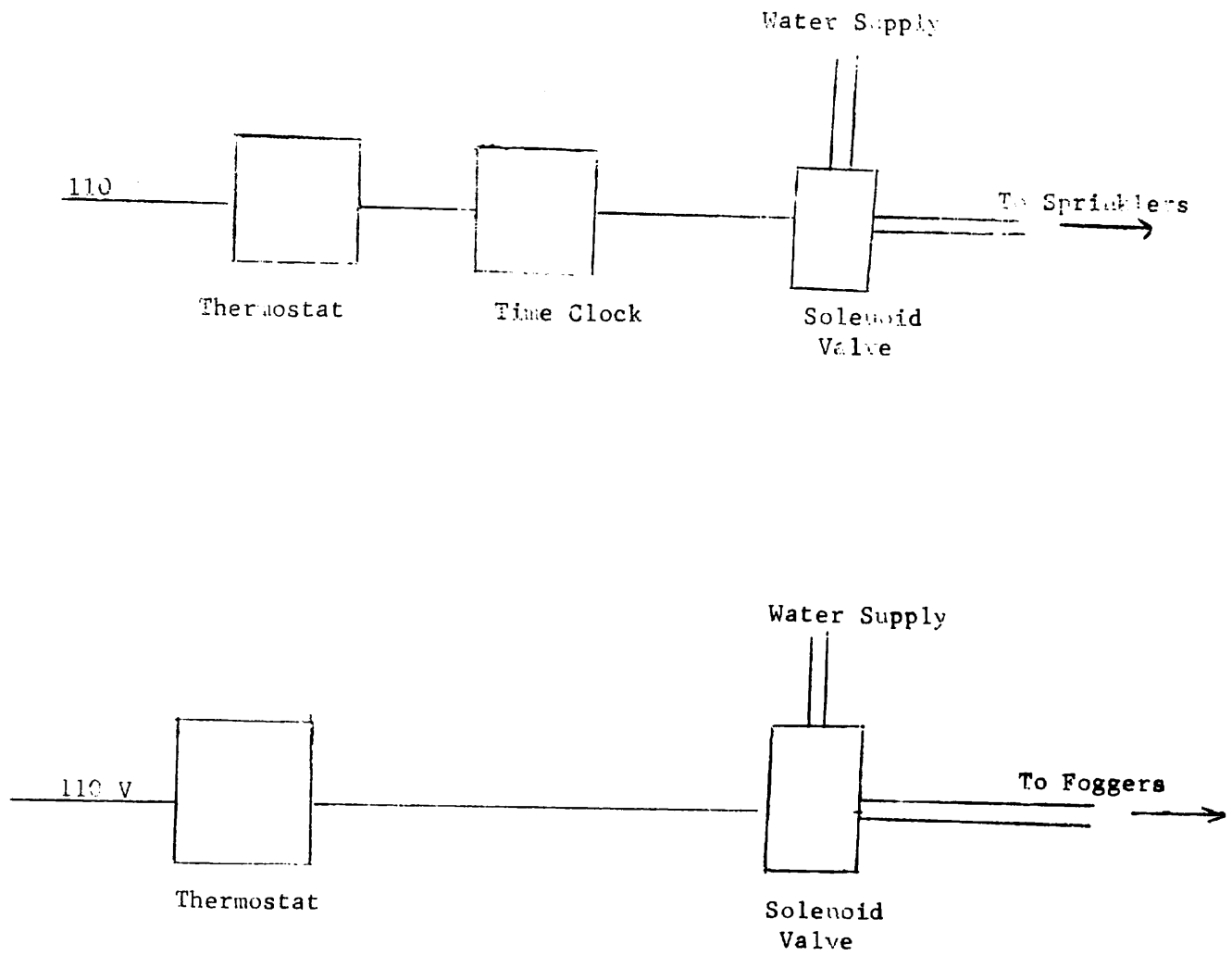
Figure 1. Control systems for sprinklers and foggers
