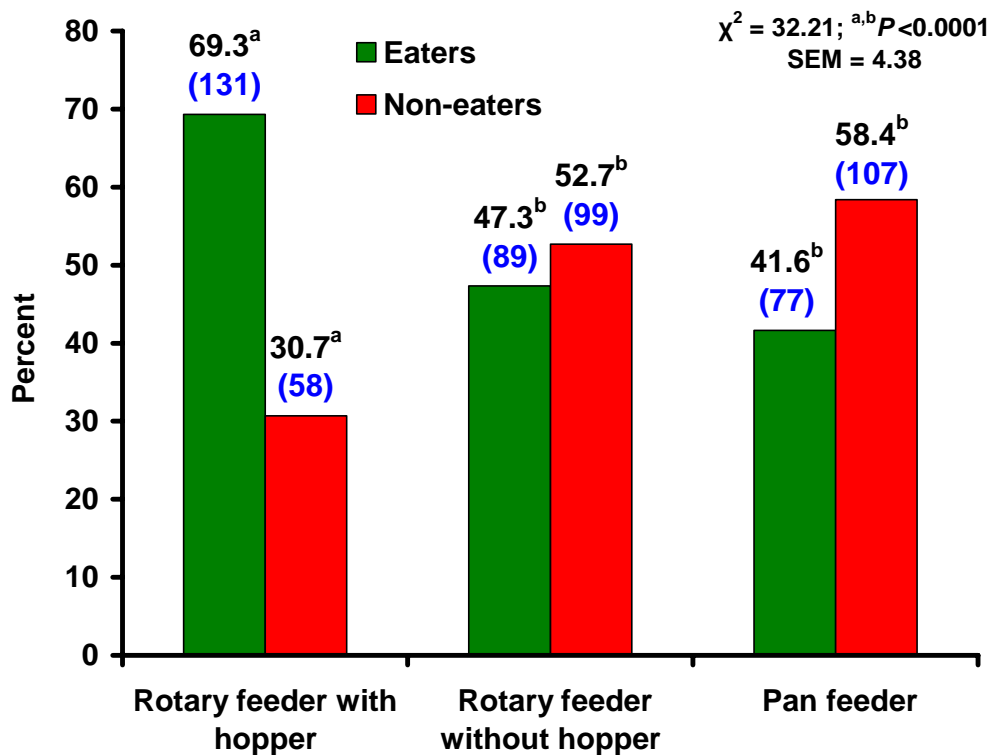
Figure 5. Effect of Creep Feeder Design on Creating Eaters (number of pigs in parentheses).
