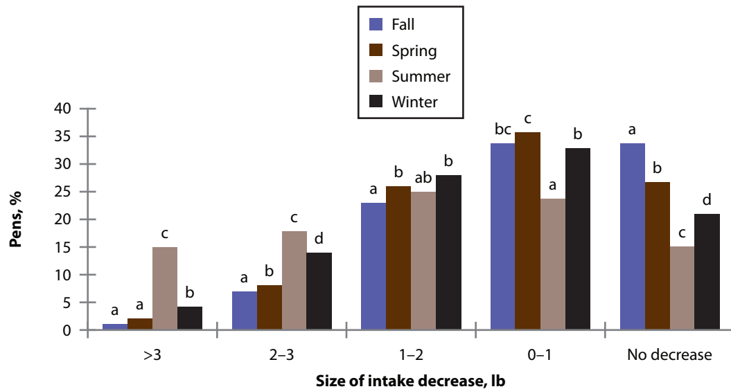
Figure 7. Percentage of pens with a decrease in DMI after initiation of zilpaterol feeding by size of decrease and season (season \times size of decrease, P < 0.01 ). Means (bars) without a common letter differ, P < 0.05 .
