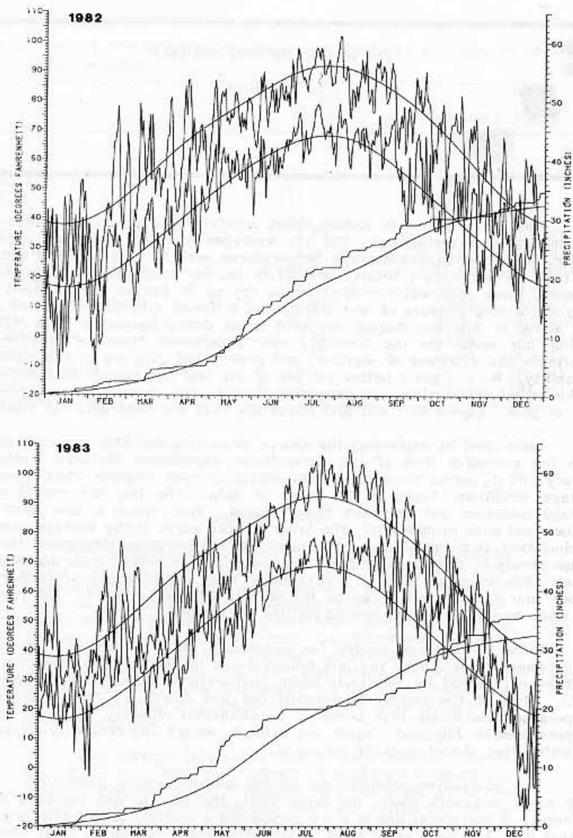
Figure 36.1. 1982 and 1983 temperature and precipitation for Manhattan, Kansas. Kansas Agricultural Experiment Station Weather Data Library.
