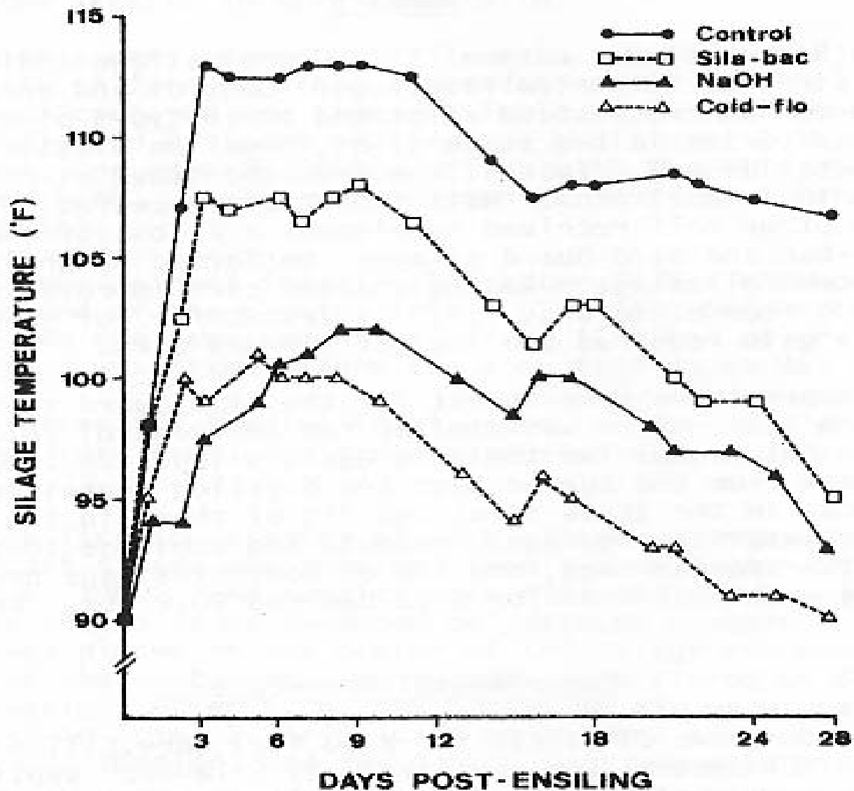
Figure 1. Ensiling temperatures for control, Sila-bac, Cold-flo, and NaOH sorghum silages (October 8-9 to November 5, 1979).
