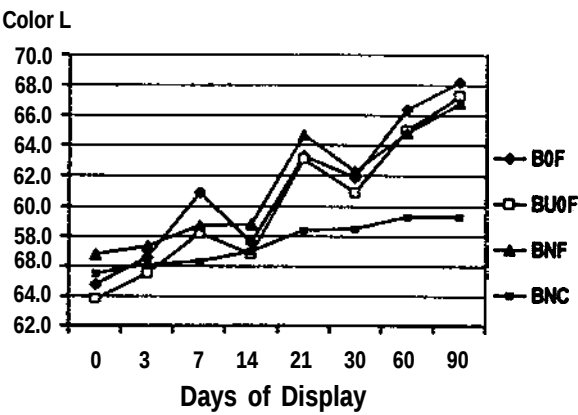
Figure 2. Color L* of Frankfurters during Display.
