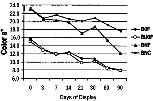
Figure 3. Color a* of Frankfurters during Display.
