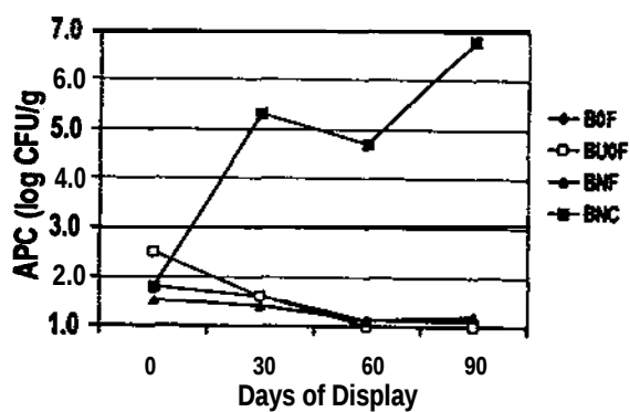
Figure 6. Aerobic Plate Count (APC) of Frankfurters during Display.
