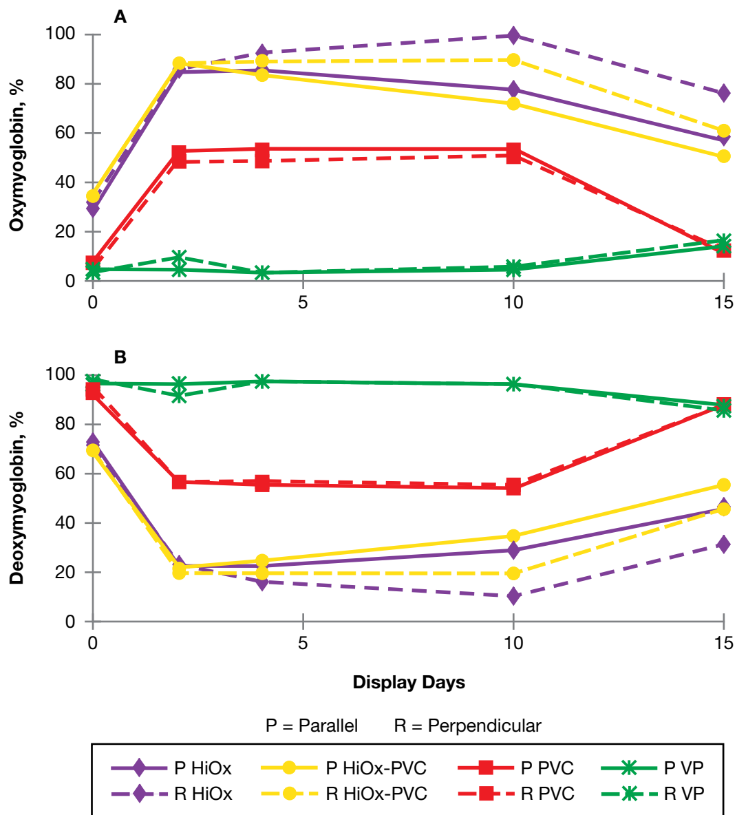
Figure 3. Packaging \times day interaction of tissue oximeter response for (A) oxy myoglobin and (B) deoxy myoglobin.
