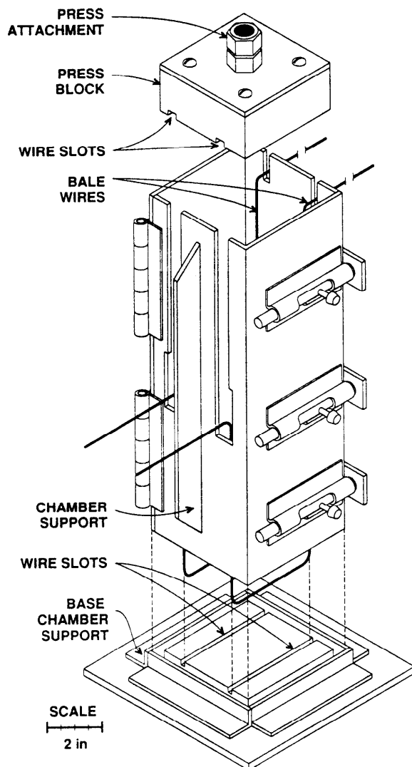
Figure 1. Scaled Drawing of the Laboratory Baling System
